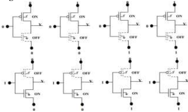
Figure 1.4 Switching activity of GDI cell
