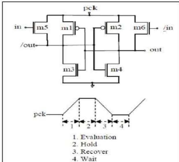
Fig. 2. PFAL Logic Circuit
