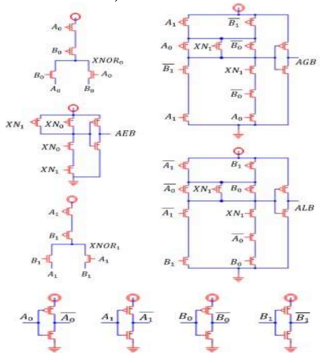
Fig. 3. Proposed 2-bit MC
