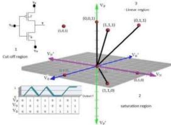
Figure 1.5 3-D operational characteristics of basic GDI cell
