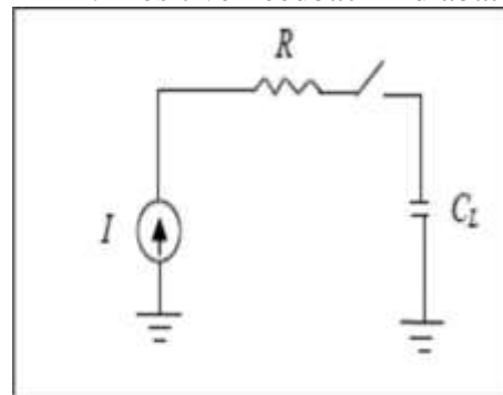
Fig. 1. Adiabatic Logic Circuit [2]
